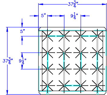
PLAN VIEW
