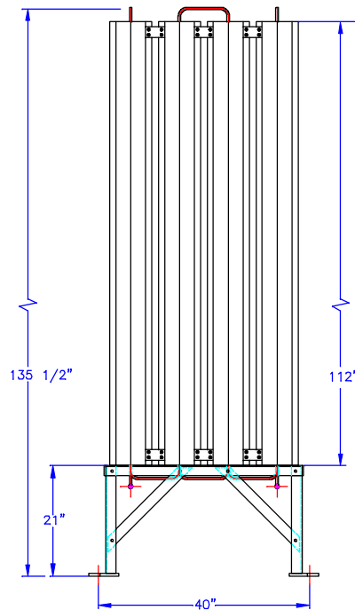
ELEVATION VIEW
