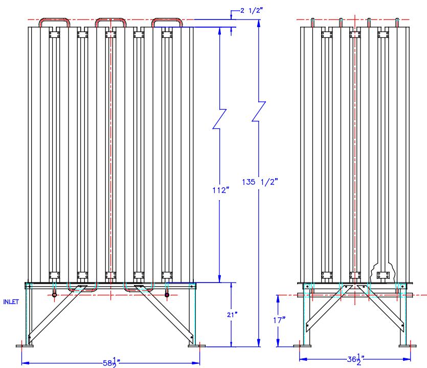
ELEVATION VIEW
